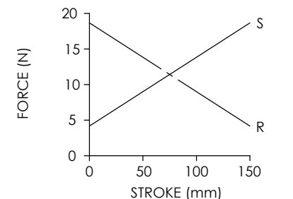
SPRING FORCE VS STROKE (CODE 'R' OR 'S' <150mm STROKE)
