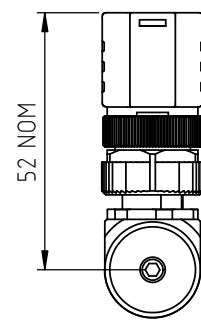
RADIAL IP67 M12 CONNECTOR IEC 61076-2-101 (CODE 'K')
