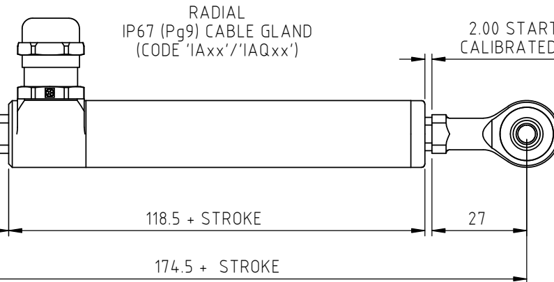
PUSH-ROD MOUNTED M5 ROD EYE (CODE 'U')
