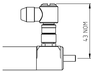
RADIAL IP67 M8 CONNECTOR IEC 61076-2-104 (CODE 'KA')
